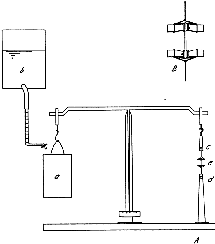
Fig. 6.— A , Apparatus used in determining breaking load of collenchyma and vascular bundles; B , detailed diagram showing method by which strands of tissue are attached.
