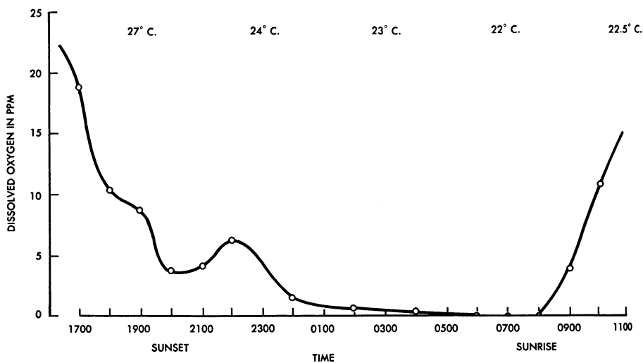
Fig. 34. Fluctuations in dissolved oxygen observed at edge of oxidation pond V at Concord, California, September 26-27, 1952.
