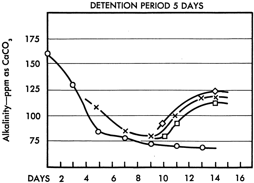
Fig. 19. Variations in total alkalinity observed in laboratory in continuous growth units.
