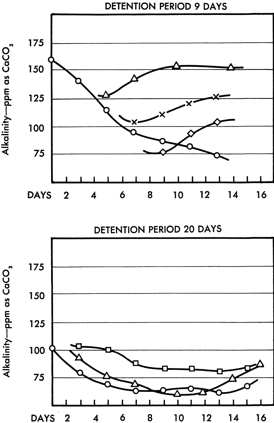
Fig. 20. Variations in total alkalinity observed in laboratory in continuous growth units.
