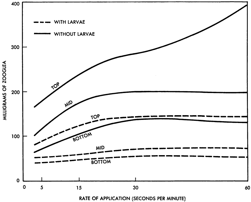
Fig. 3. Dry weight zooglea per 100 cm 2 of filter stone surface observed at Richmond pilot plant.
