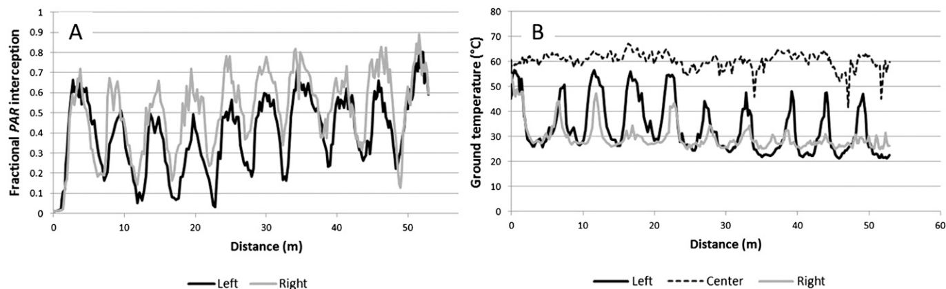
Fig. 2. Typical photosynthetically active radiation ( PAR ) interception (A) and thermal soil surface temperature (B) sensor data for a 3-year-old almond orchard ('Nonpareil' on right side of light bar and pollinizer on the left) on 15 Sept. 2010. (A) PAR interception from sensors in the left section and right sections. (B) Ground IR thermometer data for soil surface temperature underneath the 'Nonpareil' tree row canopy (left), middle of drive row (center) and underneath the pollinizer tree row canopy (right); 1 \text{ m} = 3.2808 \text{ ft} , (1.8 \times ^\circ\text{C}) + 32 = ^\circ\text{F} .
