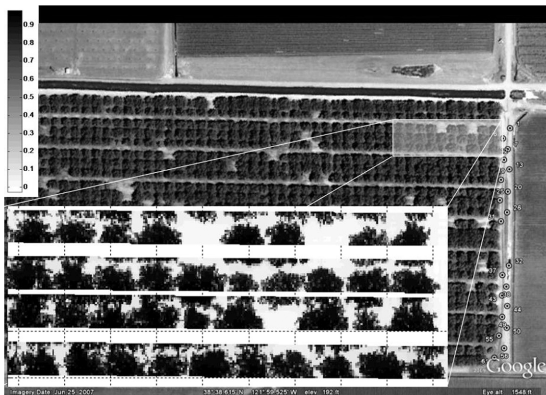
Fig. 4. An overlay of an exploded view of a small part of a walnut orchard in Yolo County, CA, showing the photosynthetically active radiation ( PAR ) absorption at 1300 HR on 10 Aug. 2009. The Google Earth map [courtesy of Google, Mountain View, CA (24 Sept. 2009)] is shown in the background. The grayscale image is a two-dimensional plot of the ratio of absorbed PAR to incoming PAR above the canopy. The darker regions represent heavy absorption implying higher canopy PAR interception. The exploded view was generated using MATLAB (MathWorks®, Natick, MA); 1 ft = 0.3048 m.
