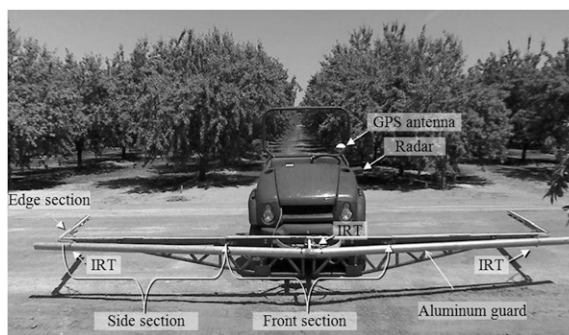
Fig. 1. Mobile platform measurement system retrofitted on a utility vehicle (model 610 Mule; Kawasaki Heavy Industries, Tokyo) for measurement of photosynthetically active radiation (PAR) interception in orchards; IRT = IR thermometers, GPS antenna = global positioning satellite receiver antenna.
