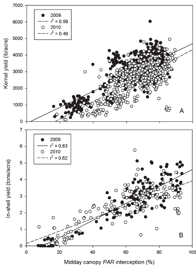
Fig. 8. Midday canopy photosynthetically active radiation ( PAR ) interception vs. yield for all almond (A) and walnut (B) sites in 2009 and 2010. Almond yield data are expressed as kernel pounds per acre and walnut as in-shell tons per acre since this is how the growers are compensated. Equations for lines for all data for almond 2009 ( y = 48.1x + 104.2 ), almond 2010 ( y = 52.3x - 893.5 ), walnut 2009 ( y = 0.051x - 0.514 ), and walnut 2010 ( y = 0.038x + 0.139 ). To test if unbalanced design was influencing regression lines, equations were also calculated for mean site data. Equations for lines with mean site data are almond 2009 ( y = 7.5x - 169.9 ), almond 2010 ( y = 45.3x - 700.3 ), walnut 2009 ( y = 0.050x - 0.611 ), and walnut 2010 ( y = 0.034x + 0.279 ); 1 lb/acre = 1.1209 kg·ha -1 , 1 ton/acre = 2.2417 Mg·ha -1 .
