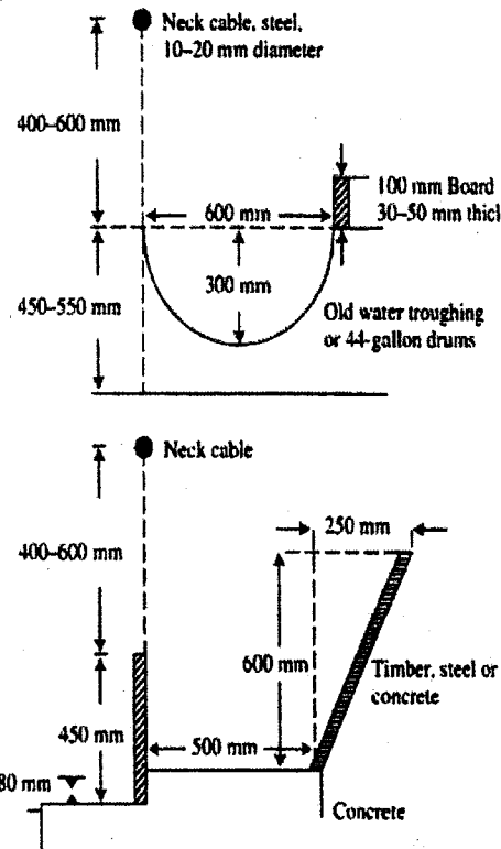
Figure 9. Two designs of feed troughs, situated outside the feedlot. Cattle eat by reaching through an opening in the fence
