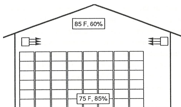
Figure 1. Curing room with top mounted heaters. Numbers in boxes are typical air temperature and relative humidity in the top and bottom portions of the room.
