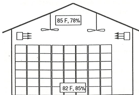
Figure 2. Curing room with top mounted heaters and ceiling fans. Numbers in boxes are typical air temperature and relative humidity in the top and bottom portions of the room.
