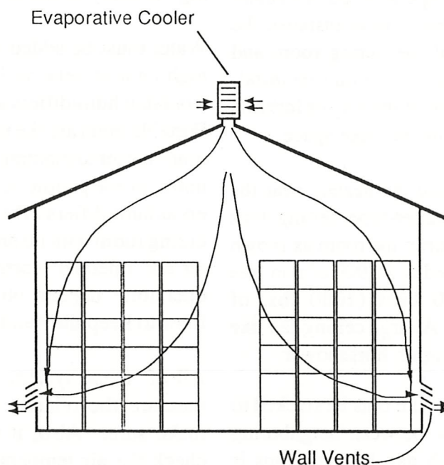
Figure 3. Air flow in an evaporatively cooled sweetpotato storage room
