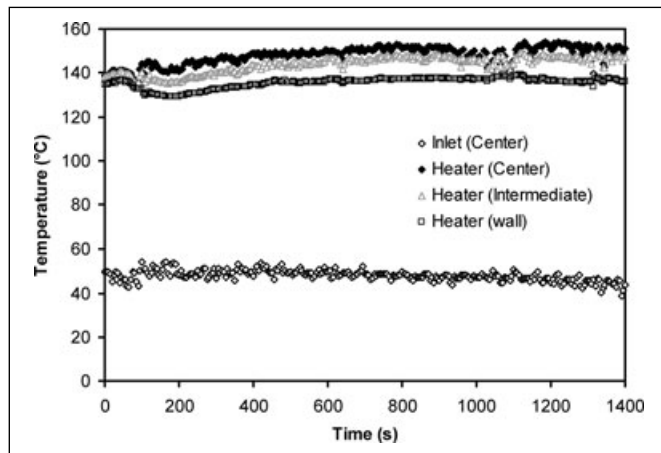
Figure 4 – Typical time-temperature history at the inlet of the microwave heating section and outlet of 2nd microwave applicator (Run 1).
