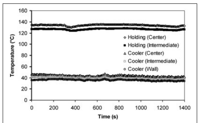
Figure 6 – Typical time-temperature history at the exit of the holding and cooling sections (Run 2).
