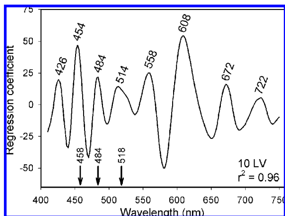
Figure 3. Regression coefficients for prediction of lycopene content from the visible spectrum (410–750 nm). Data smoothed with the Savitzky–Golay algorithm (11 nm range, second-order polynomial). LV, latent variables. Arrows indicate peak absorption of pure lycopene in chloroform (31).
