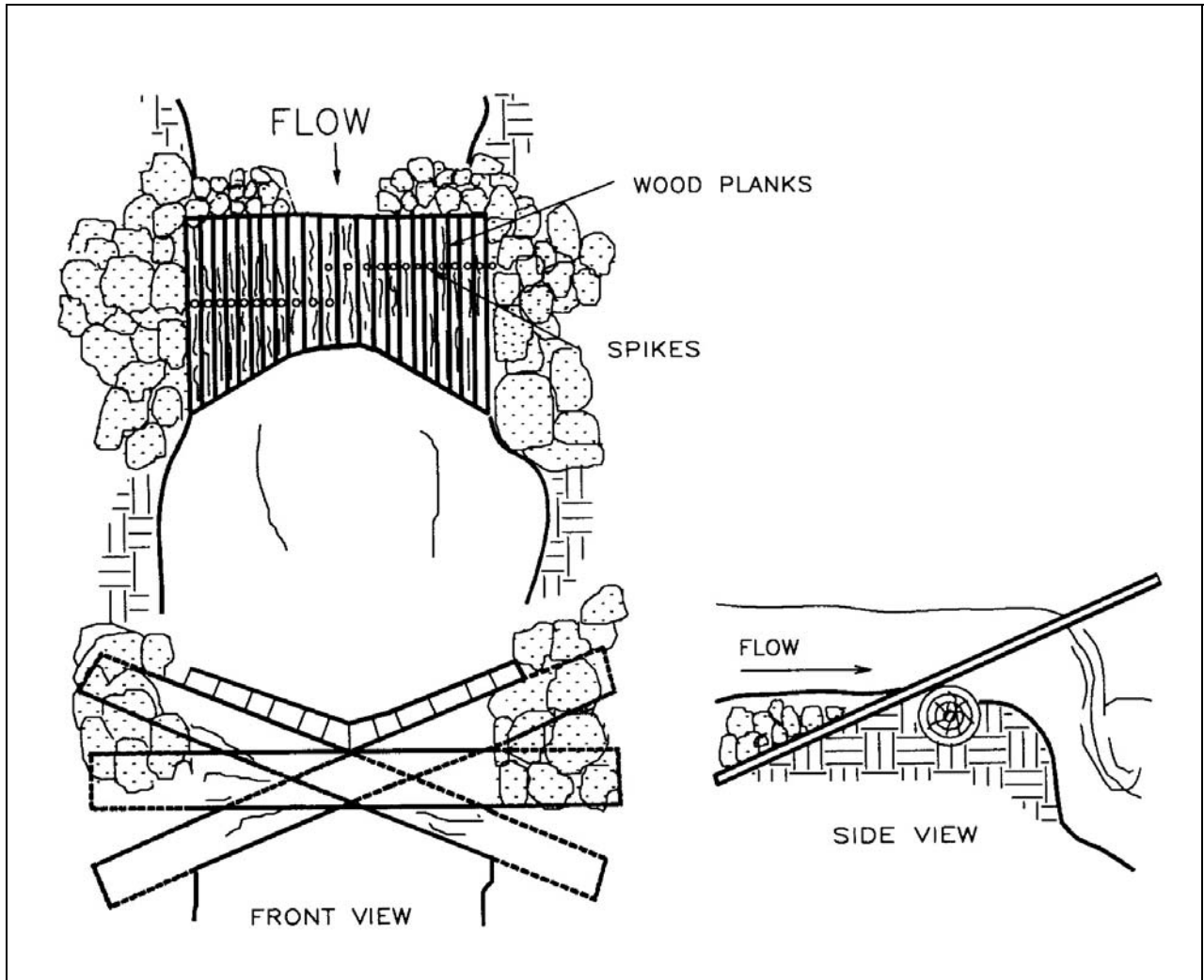
Figure VII-36. Hewitt ramp.
