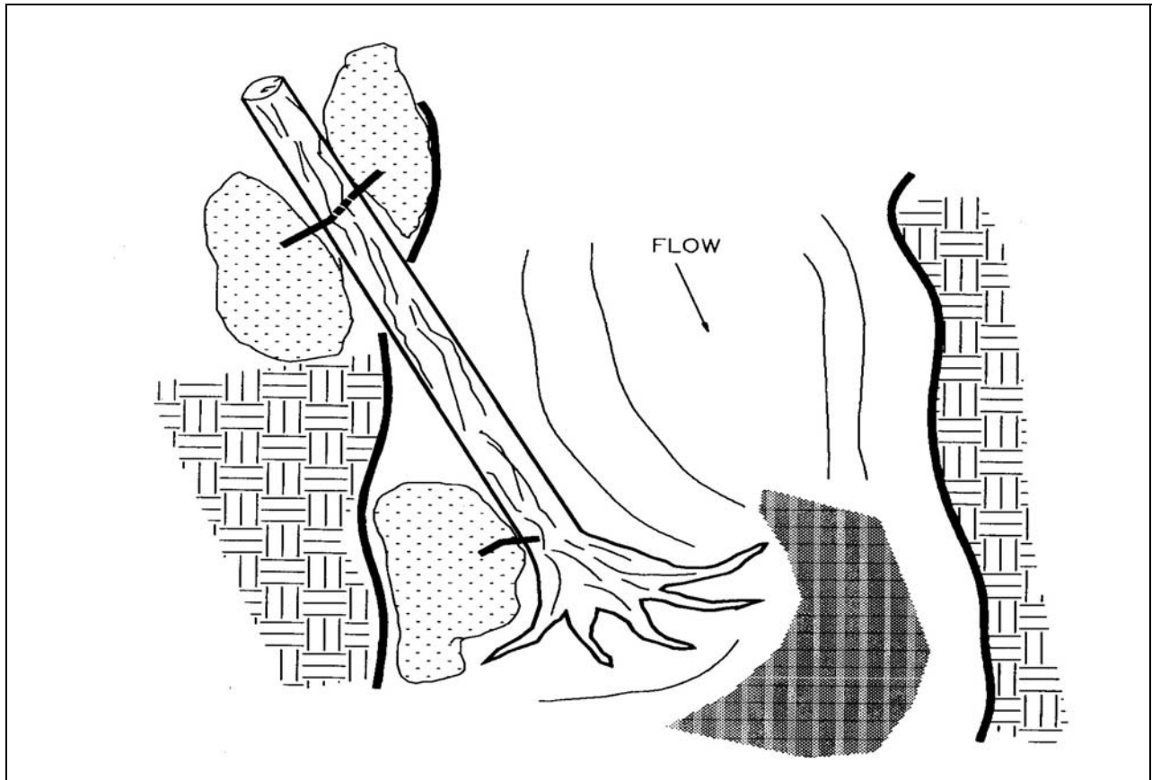
Figure VII-18. Digger log.
