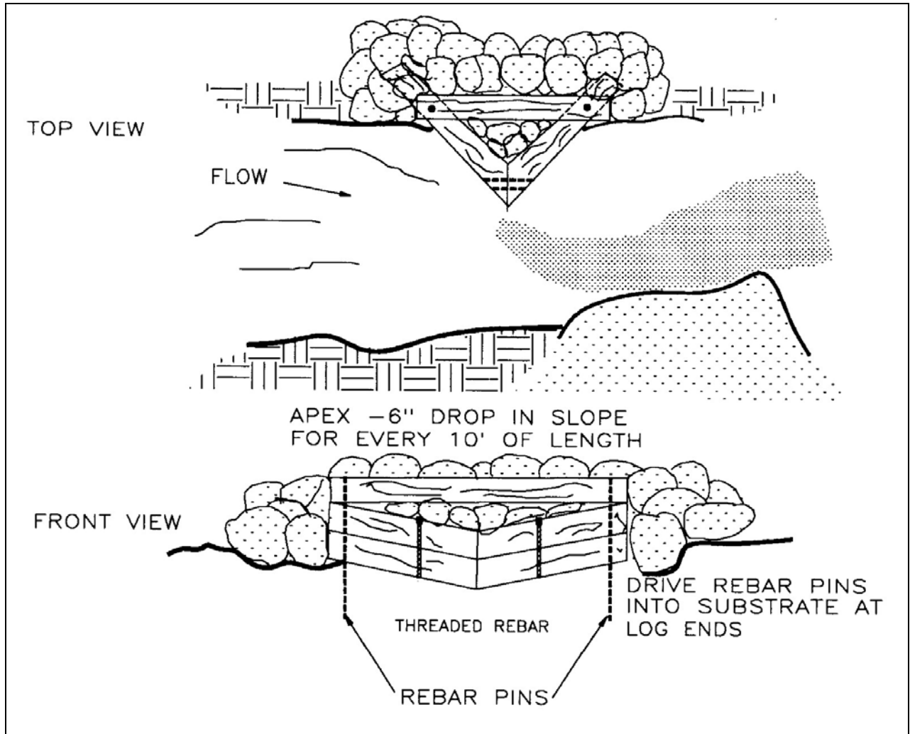
Figure VII-53. Log wing-deflector.
