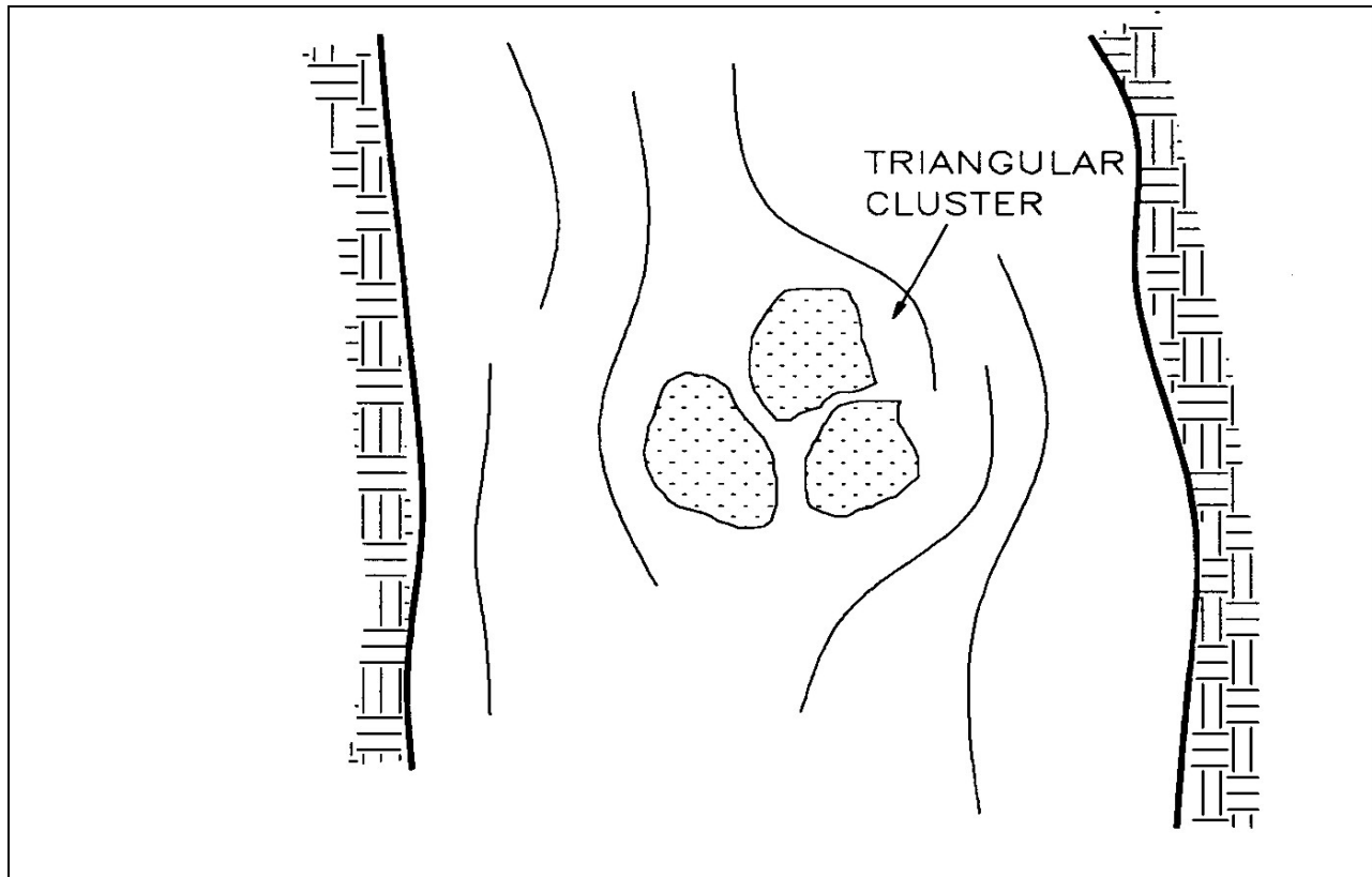
Figure VII-25. Boulder cluster.
