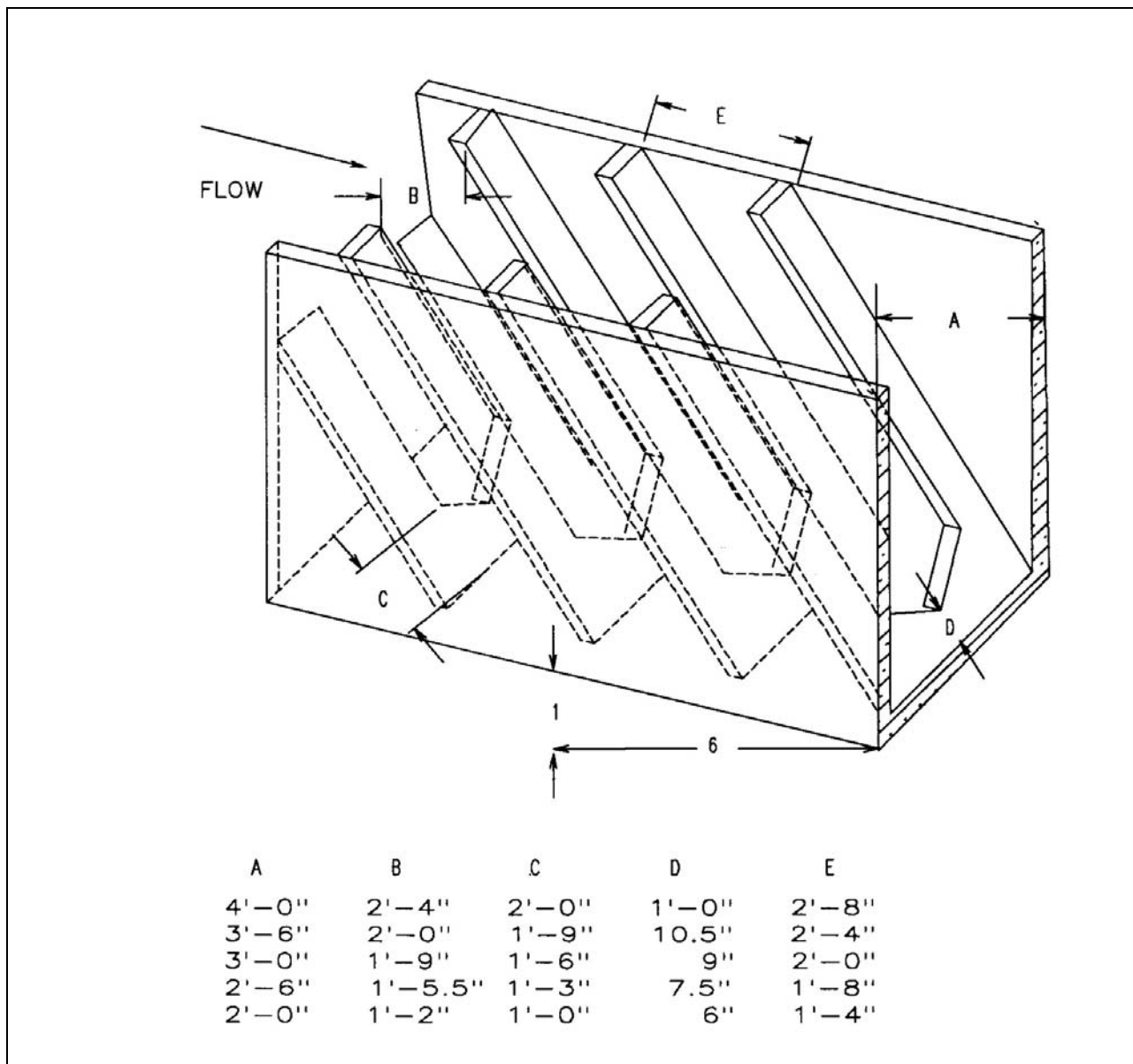
Figure VII-40. Denil fishway.
