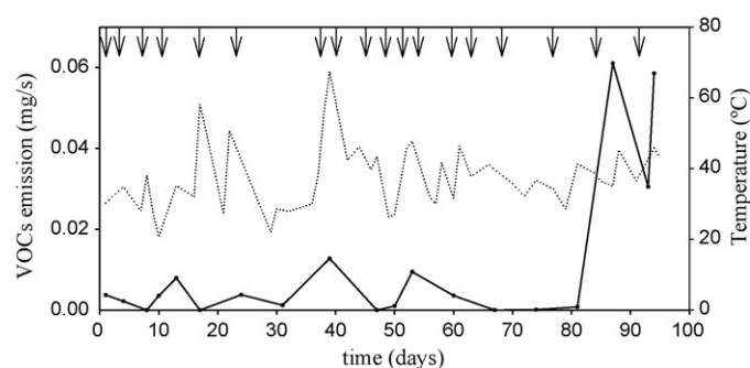
Fig. 4. VOCs emissions during home composting (solid line). The temperature profile is also shown (dotted line). Upper arrows represent the organic material loads to the composter.
