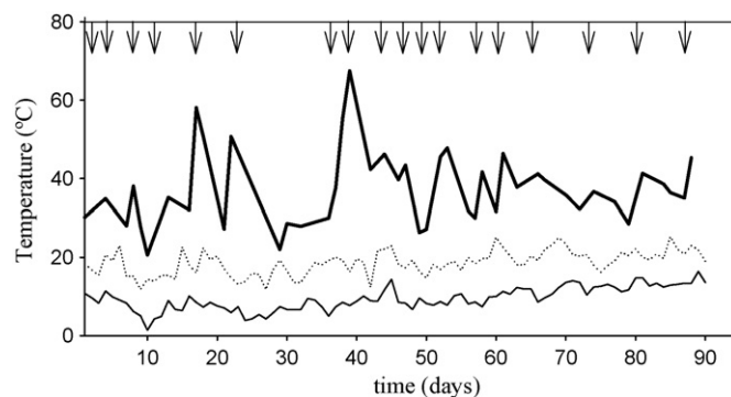
Fig. 3. Temperature profiles. The bold solid line (—) represents the temperature profile of the composter. The thin solid (—) and dotted lines (···) represent the minimum and the maximum ambient temperatures, respectively. Upper arrows represent the organic material loads to the composter.
