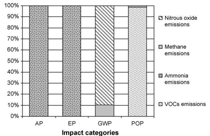
Fig. 6. Contribution (in percentage) of each gas contaminant ( N_2O , CH_4 , NH_3 and VOCs) to the total environmental impact of the gaseous emissions of home composting for the impact categories affected (AP, EP, GWP and POP). Data is referred to the initial scenario. Impact categories: AP, acidification potential; EP, eutrophication potential; GWP, global warming potential; POP, photochemical oxidation potential; CED, cumulative energy demand.
