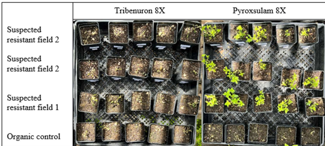
Figure 4. ALS inhibitor herbicide to control chickweed in a greenhouse study. Plants from suspected resistant fields were reduced and some killed by tribenuron at 8X the label rate, although lower rates did not control the weed as well. Plants from suspected resistant fields were not controlled or killed by pyroxsulam up to 8X the label rate.
