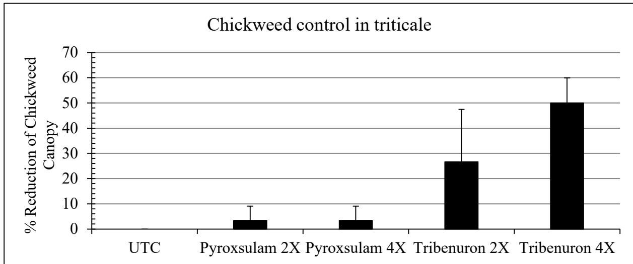
Figure 3. Results from in-field herbicide rate study on chickweed control. Tribenuron showed some activity by reducing the chickweed canopy but pyroxsulam did not. Error bars represent one standard deviation. Bars under the same lowercase letter are not significantly different at \alpha = 0.05 according to a Tukey HSD test.
