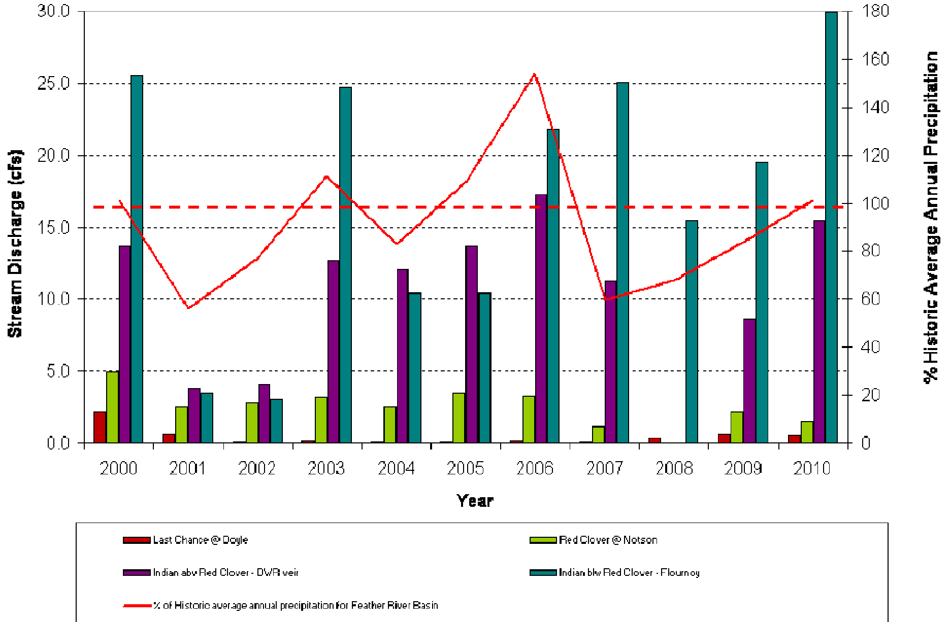
Weekly Average Minimum Flows 2000-2010 on Last Chance Creek and Red Clover Creek and Indian Creek above and below the confluence of Red Clover Creek
