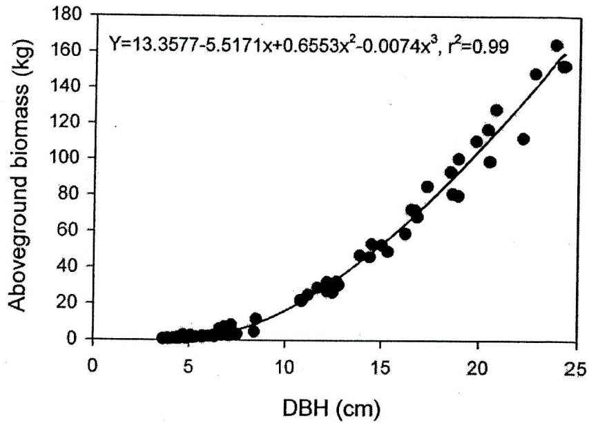
Figure 1—Ponderosa pine diameter-based biomass regression for 21-yr-old trees at Whitmore and some small diameter trees harvested at the Long-Term Soil Productivity installation in northern California. The range of DBH is between 3.6 cm and 24.3 cm.
