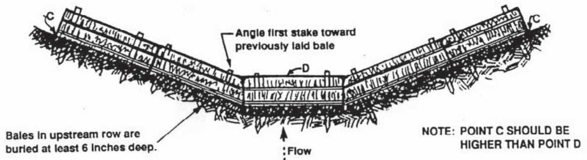
Section B-B
