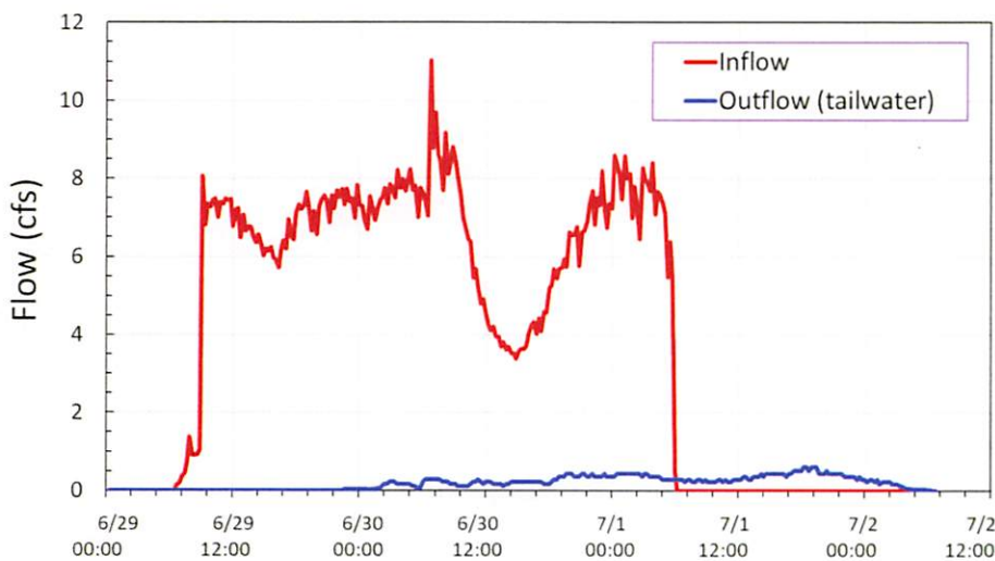
Fig. 2. Inflow rate and tailwater runoff rate over an irrigation event in a klein grass field equipped with automated surface irrigation.
