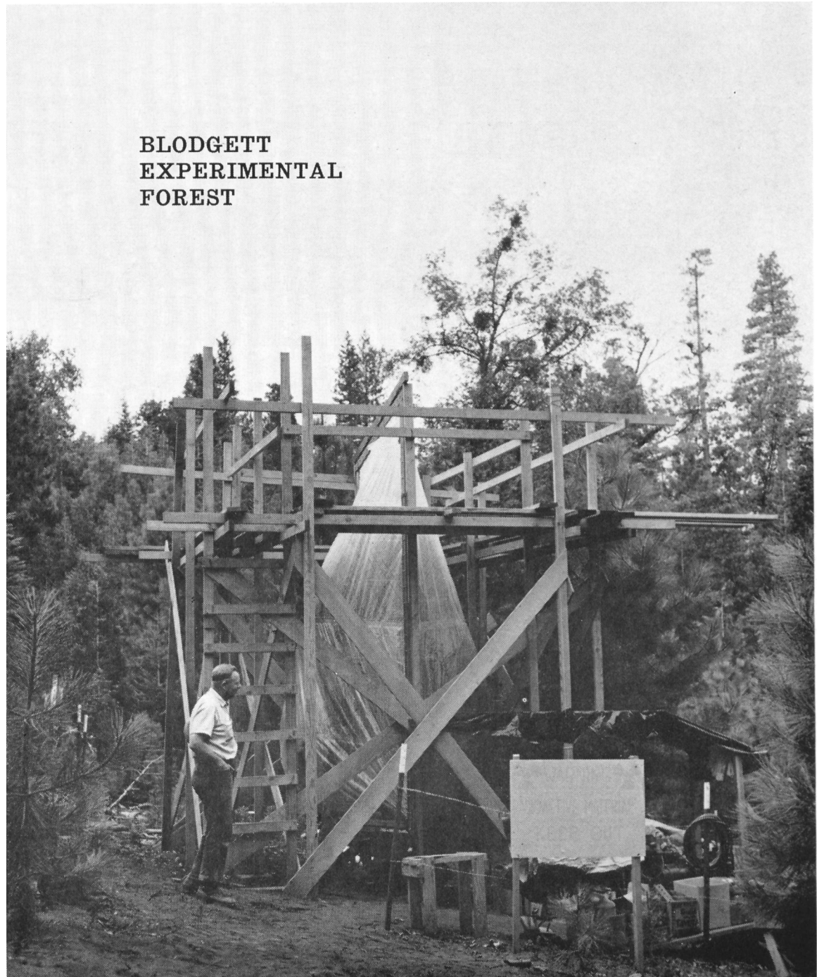
Plastic-enclosed pine tree at Blodgett Experimental Forest, El Dorado County, is being treated in an artificial atmosphere to obtain radioactive resin for use in studies of resin production, as it may affect insect resistance →
