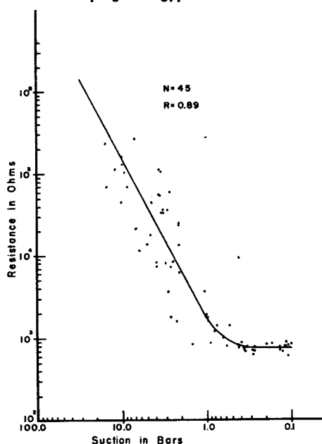
Calibration curve for Bouyoucos resin-impregnated gypsum blocks.
