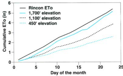
Fig. 2. Cumulative ETo from La Conchita Ranch evaporation pans and from Rincon stations ETo during August 1996.
