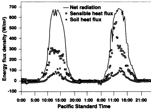
Fig. 1. Bowen ratio tower energy flux density at La Conchita Ranch for mature lemons, Aug. 3 and 4, 1998.
