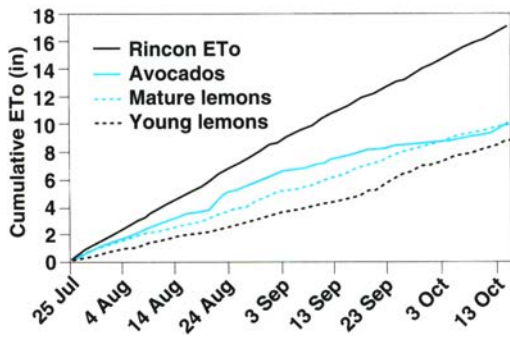
Fig. 4. Cumulative ETo measurements in different orchards at La Conchita Ranch as compared to Rincon ETo.
