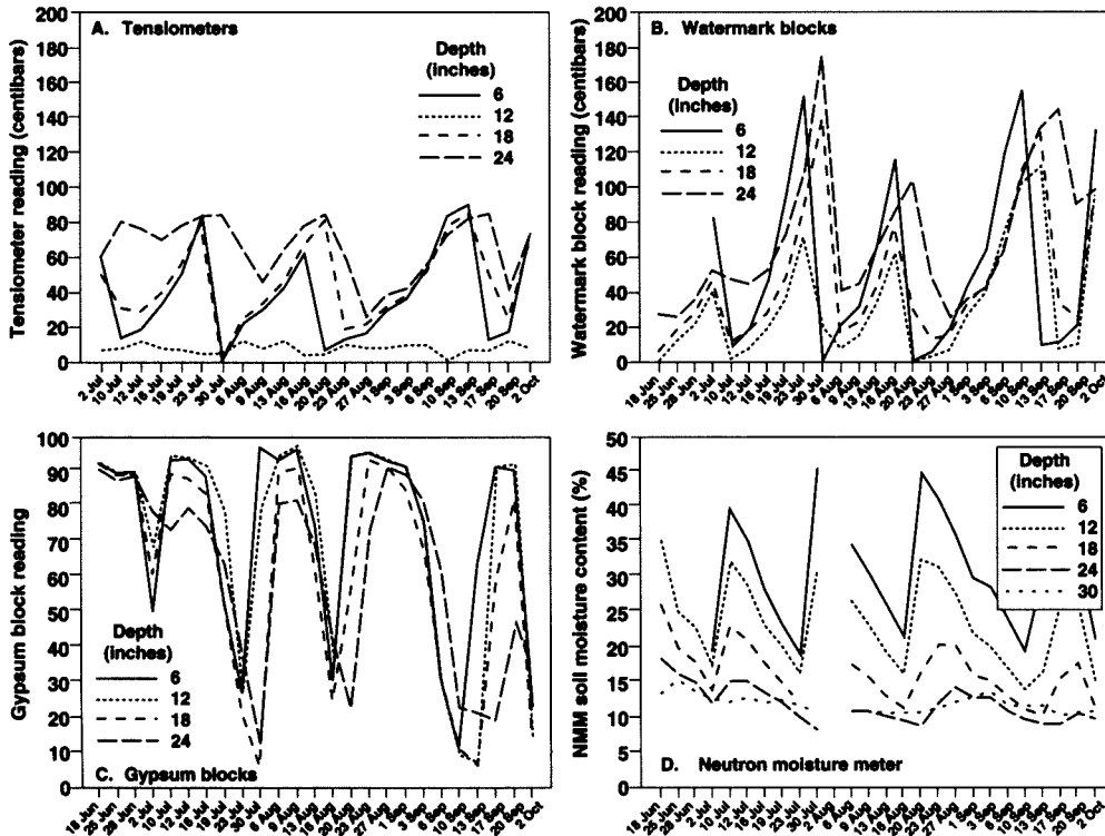
Fig. 1. Tensiometer readings (A), Watermark block readings (B), gypsum block readings (C) and NMM volumetric soil moisture contents (D) with time during irrigation season for a food-irrigated walnut orchard grown in a sandy loam soil.
