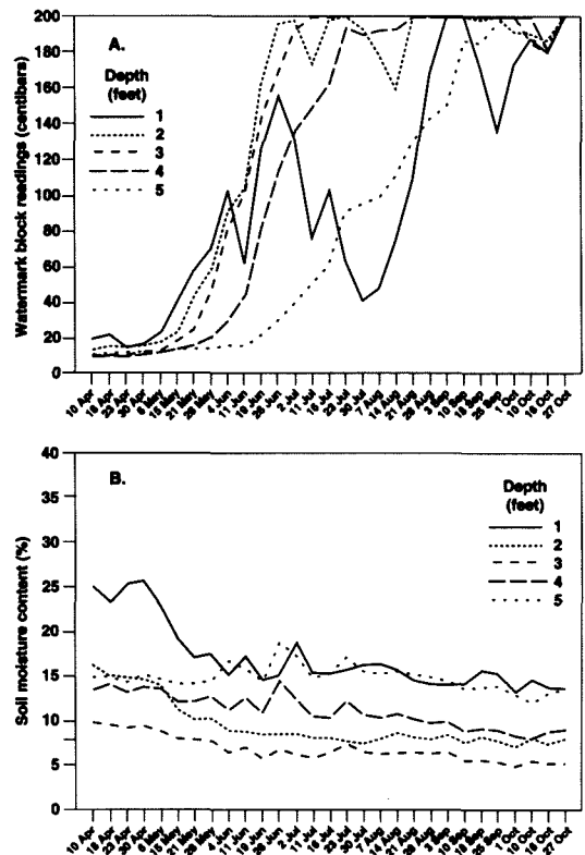
Fig. 3. Watermark block readings (A) and NMM volumetric soil moisture contents (B) with time during the irrigation season for center-pivot-irrigated alfalfa.
