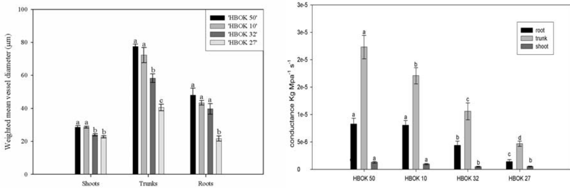
Figure 2. Weighted mean xylem vessel diameter and calculated theoretical axial xylem conductance of root, trunk and shoot xylem tissue from HBOK50, HBOK 10, HBOK 32 and HBOK27 rootstocks.
