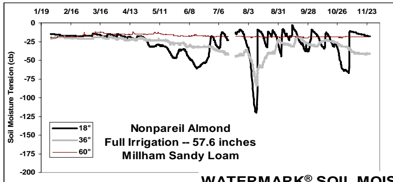
Fig. 2. Soil moisture water content (upper charts, inches/ft and % available) and soil moisture tension (lower charts, centibars as recorded by Watermark blocks) for Nonpareil trees in a mature block irrigated with micro sprinklers. Charts contrast soil water storage for the “Full” irrigation treatment (left) @ 57.6 inches with a 25% “Reduced” irrigation (right) @ 47.1 inches. The center table lists yields by irrigation and applied N.
