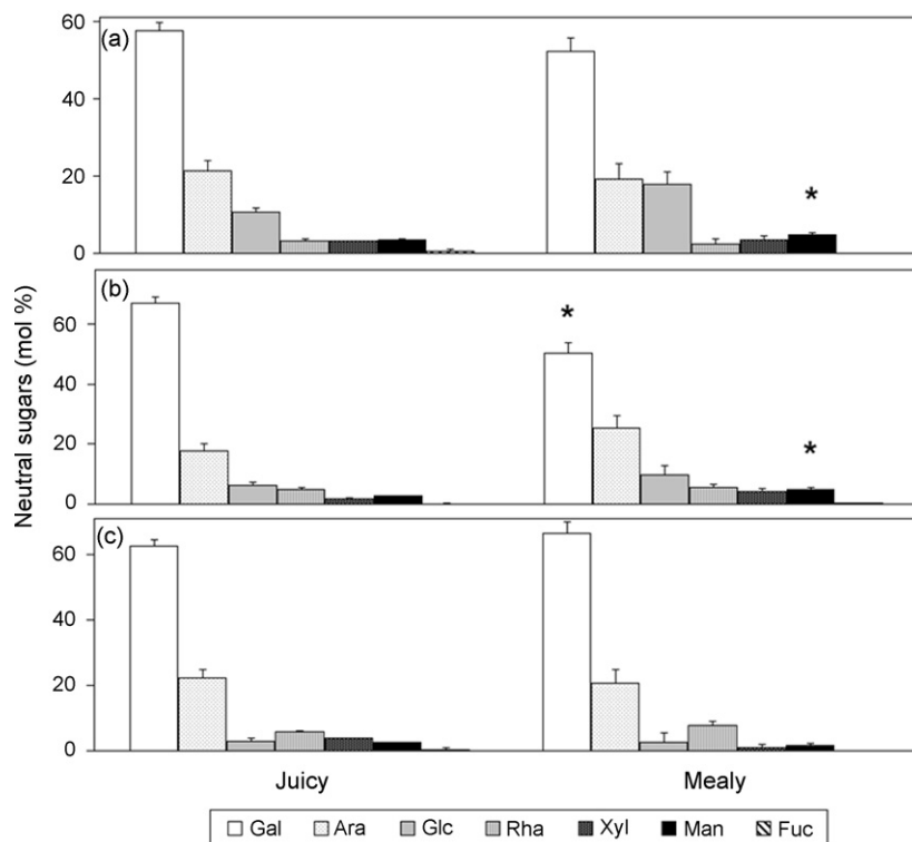
Fig. 4. Neutral sugar composition in the (a) WSF, (b) CSF and (c) NSF pectins of normally ripening (juicy) and chilling-injured (mealy) 'Fortune' plums.
