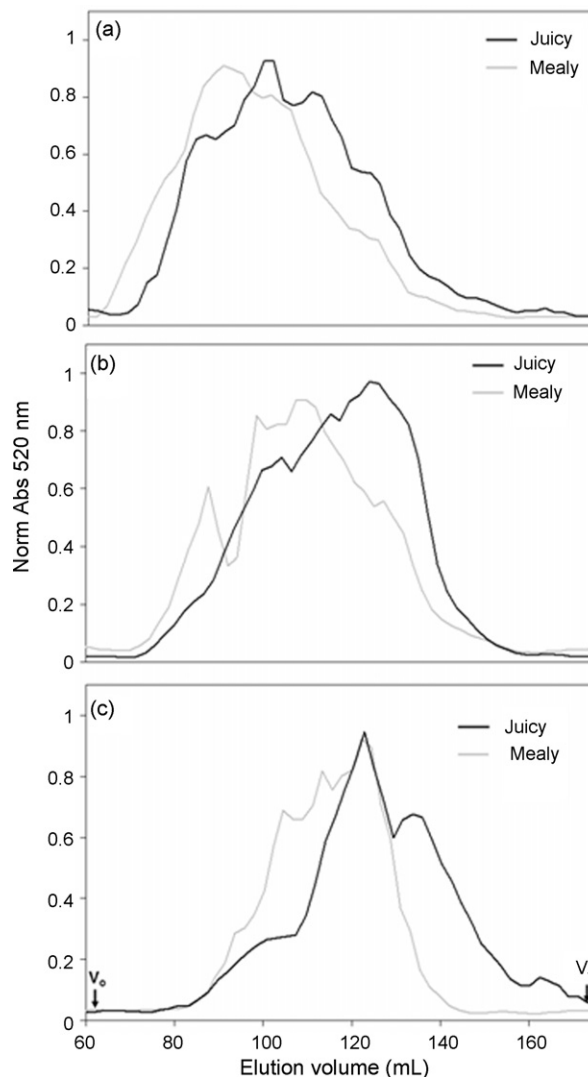
Fig. 3. Size exclusion chromatography profiles of pectin polymers of juicy and mealy 'Fortune' plums. The samples were fractionated on HW65. Column fractions (2 mL) were assayed for uronic acid content. V_0 : void volume; V_t : total volume. (a) WSF; (b) CSF; (c) NSF.
