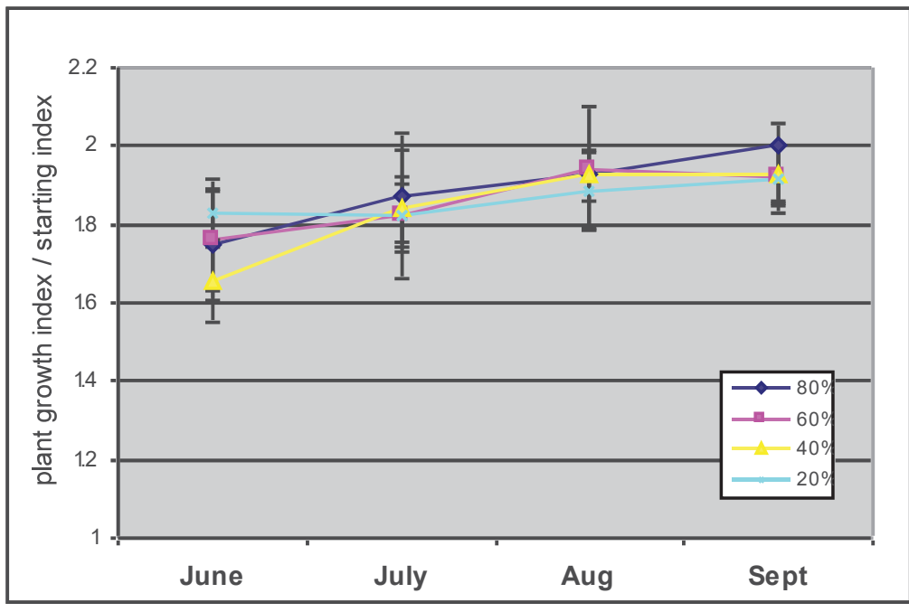
Figure 4b. Eyelash grass relative summer growth
