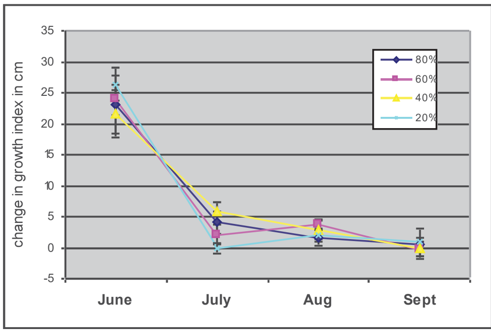
Figure 4a. Eyelash grass change in summer growth index under 4 irrigation percentages of ETo
