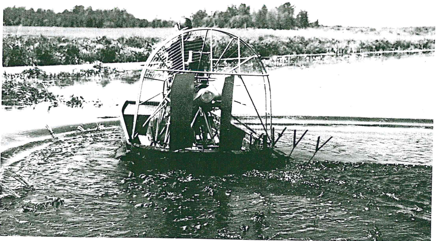
Figure 14. The v-shaped knives attached to the airboat are lowered into the water to remove rows of plants while the airboat skims across the field.
