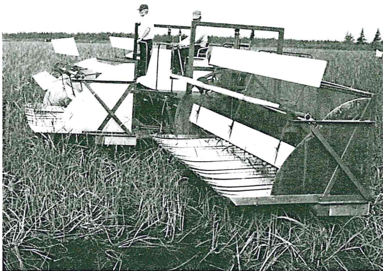
Figure 21. Multiple-pass harvester used to harvest shattering types of wild rice. The machine does not cut off the plants but only dislodges the mature kernels.
