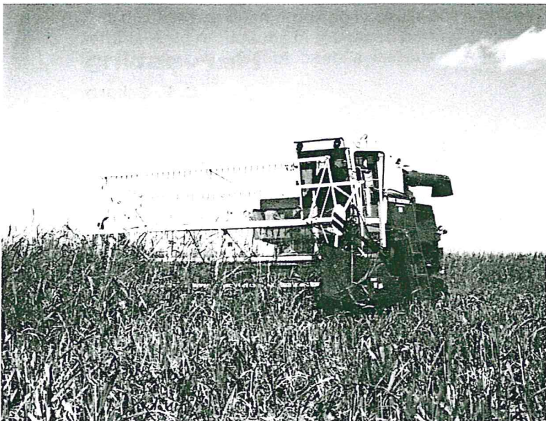
Figure 22. Harvesting wild rice with a modified rice combine.
