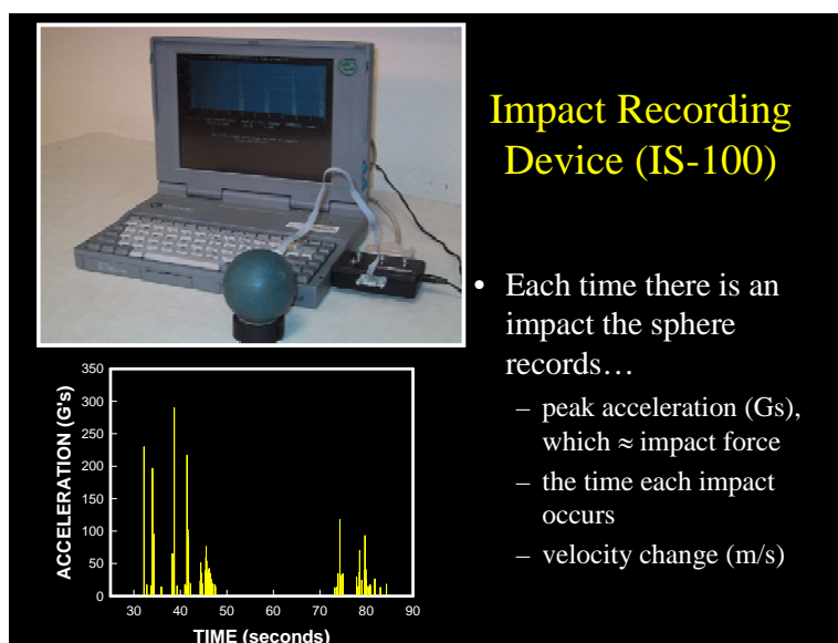
Picture 2. Accelerometer (IS-100) device used to measure impact bruising potential during packing operation.
