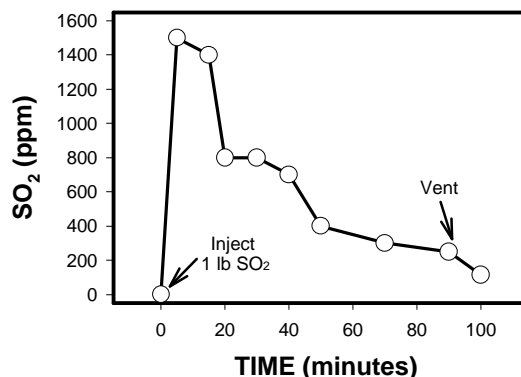
Fig. 1. Sulfur dioxide concentrations measured with Kitagawa tubes in a 2.377 ft 3 marine container after fumigation with one pound of gas.
