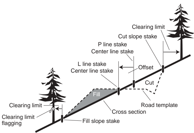
Figure 5-5. Example L-line design road section, construction-staked.
