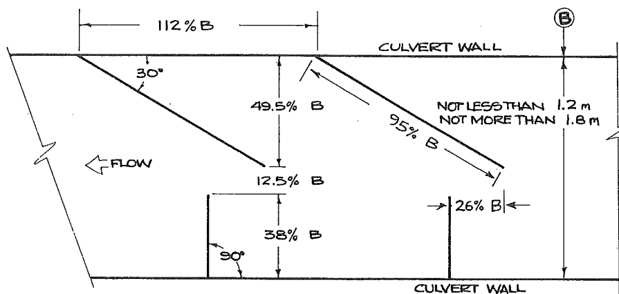
FIGURE 8.15.—Baffle design recommended by the U.S. Forest Service for culverts. Dimensions are scaled (as percentages) to culvert width ( B ), which can range from 1.2 to 1.8 m. (After Evans and Johnston 1980.)
