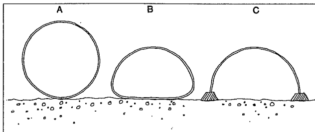
FIGURE 8.11.—Types of metal culverts used on western forest and rangeland roads: (A) corrugated-round; (B) corrugated pipe-arch; (C) structural plate-arch with concrete footings.
