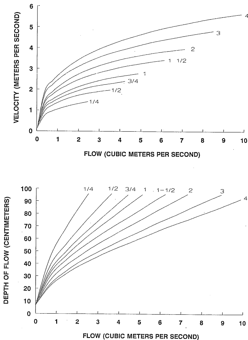
FIGURE 8.14.—Velocity-flow and depth-flow curves (U.S. Forest Service) for water flowing through a 2.1-m \times 1.6-m metal pipe-arch. Curves represent gradients of 0.25, 0.5, . . . , 4%. (After Evans and Johnston 1980.)
