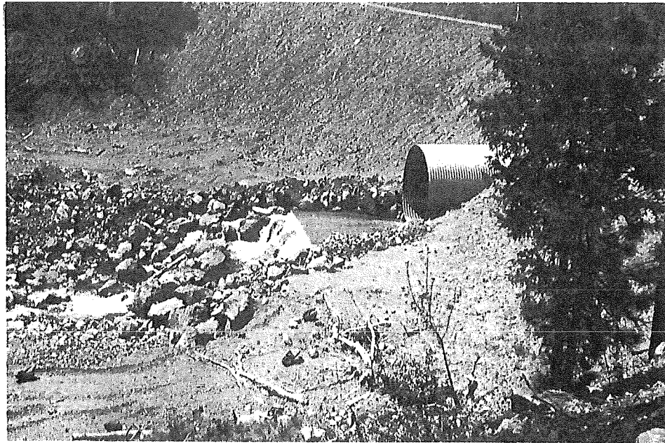
FIGURE 8.12.—Culverts installed above the grade of a stream can be a barrier to upstream fish migration. The culvert shown here is impassable to salmon and steelhead.
