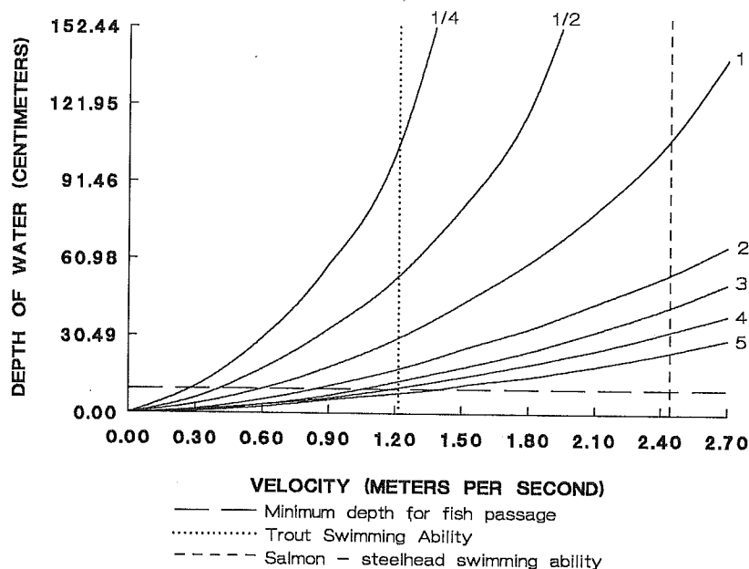
FIGURE 8.13.—Depth-velocity curves (Oregon State Game Commission 1971) for water flowing through a round, 1.8-m-diameter culvert. Curves represent gradients of 0.25, 0.5, . . . , 5%.
