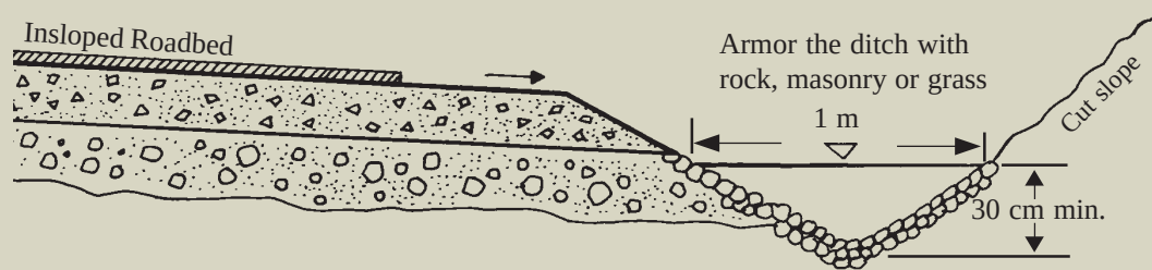
b. Typical Ditch Armoring and Shape
