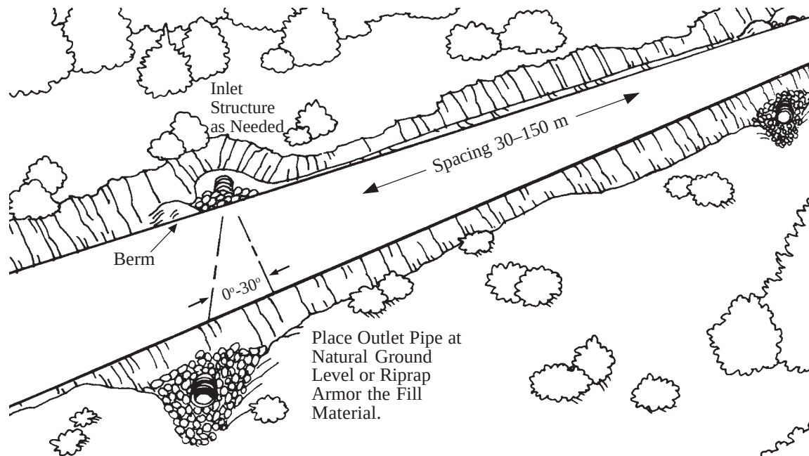
Figure 7.5 Water bar construction. (Adapted from Wisconsin's Forestry Best Management Practices for Water Quality. 1995, Publication FR093, Wisconsin Department of Natural Resources)
