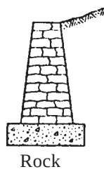
Figure 11.4 Construction of various types of retaining structures. (Adapted from Gray & Leiser, 1982)
