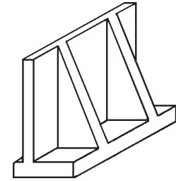
Figure 11.4 Construction of various types of retaining structures. (Adapted from Gray & Leiser, 1982)
