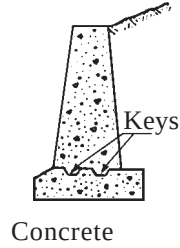
Figure 11.4 Construction of various types of retaining structures. (Adapted from Gray & Leiser, 1982)
