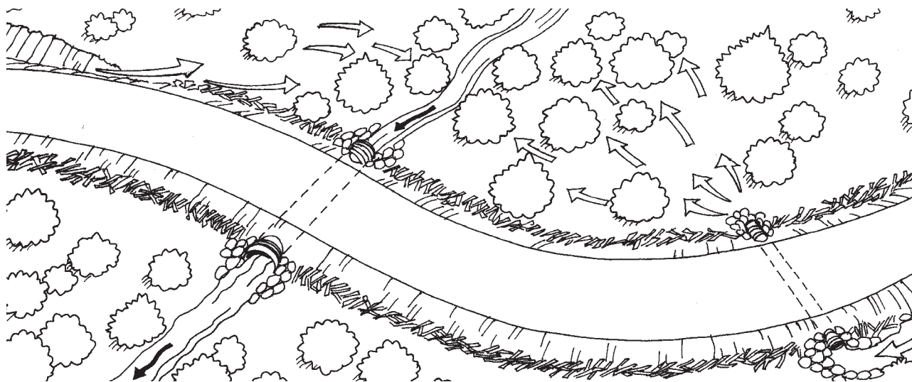
b. Basic road surface drainage with leadoff ditches and culvert cross-drains exiting into vegetation or a streamside buffer area. (Adapted from Montana State Univ. 1991)
