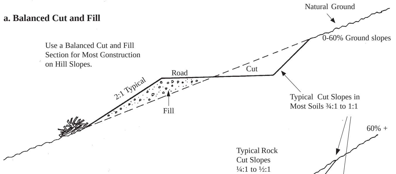
Figure 11.1 Cut slope design options.
