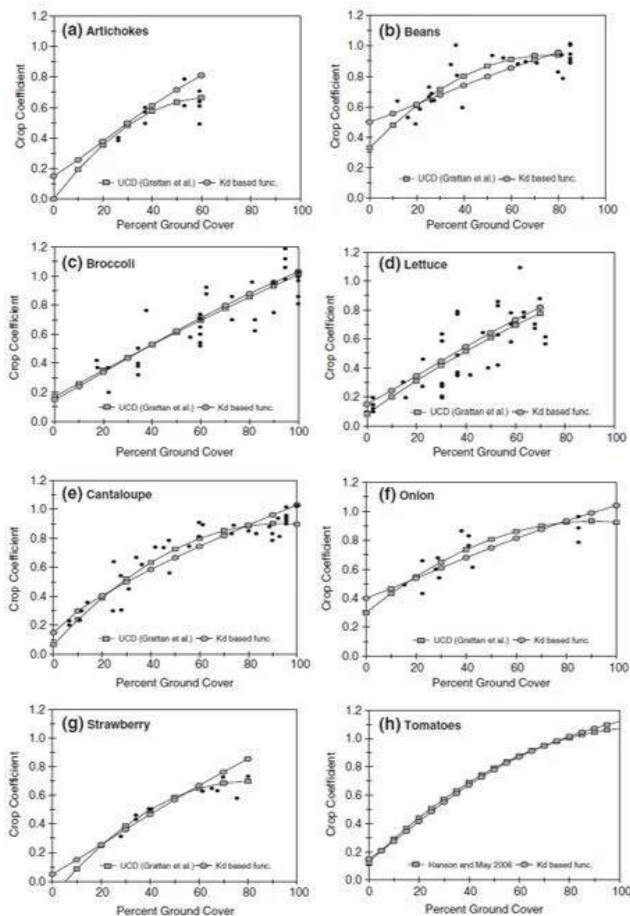
Figure 2. Examples of crop coefficients for vegetables as a function of percentage of canopy cover (from Allen and Pereira, 2009). Original caption: K c versus f c for seven vegetable crops in California reported by Grattan et al. (1998) (a–g) and tomatoes in California by Hanson and May (2006) (h), showing data and regression equations by Grattan et al. and Hanson and May (2006) with K c estimated using Eqs. 6, 7a, and 10. The small black symbols represent measured data.
