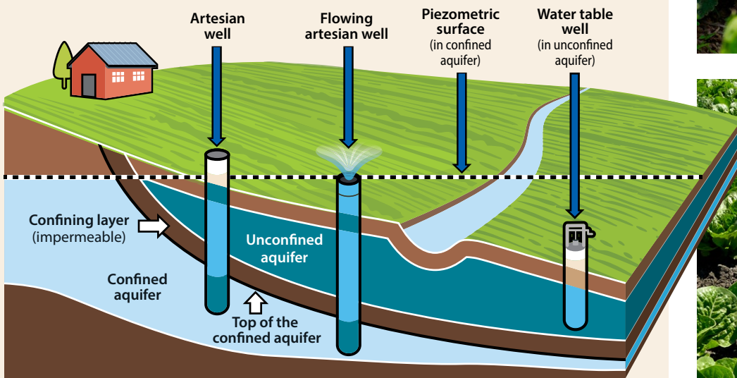
Figure 1: Groundwater flow
