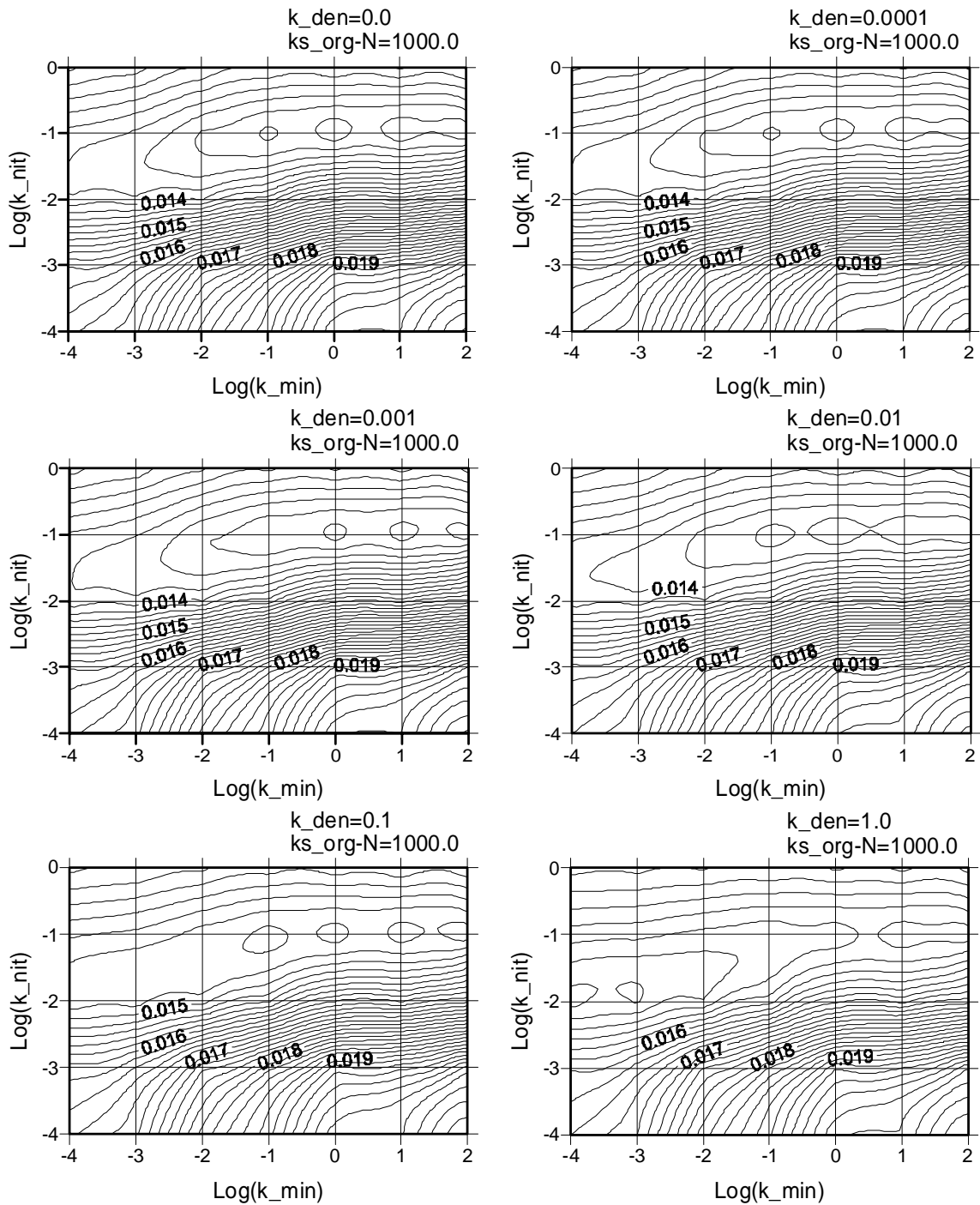
Figure 12(e): Contour maps of root mean square error between measured and calculated total \text{NH}_4\text{-N} and \text{NO}_3\text{-N} concentrations in soil ( k_{\text{org-N}} = 1000.0 ).
