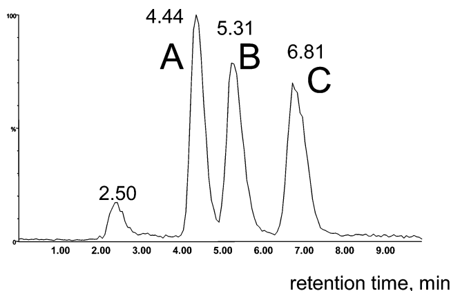
Figure 2. HPLC separation of a standard mixture under optimum conditions with MS detector (MRM mode) [5 ng/mL, 10 μL injected]. (A) Methoprene-PTAD. (B) Kinoprene-PTAD. (C) Hydroprene-PTAD.
