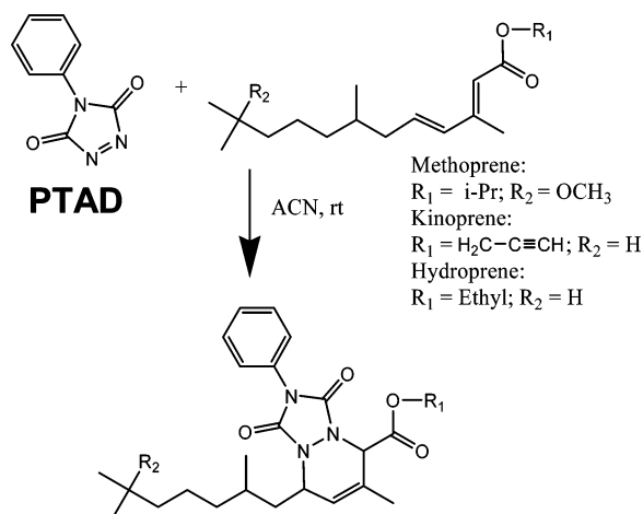
Figure 1. Derivatization reaction.
