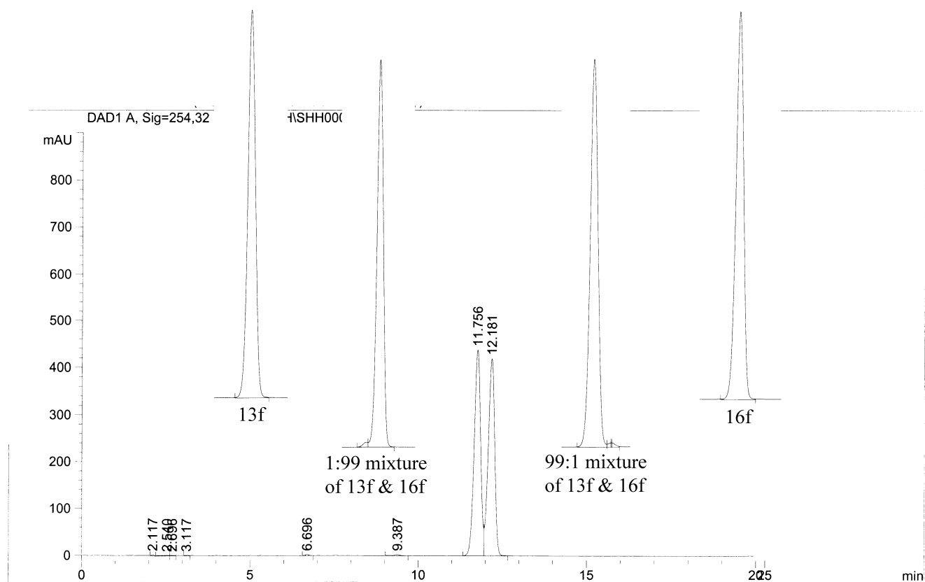
Figure 4. HPLC data for 13f and 16f . the compounds monitored at 254 nanometers with a reversed phase column (ZORBAX SB-C18, 4.6 mm x 250 mm x 5 \mu m, Hewlett Packard) running isocratically with a solvent of acetonitrile/0.1% aqueous TFA (70:30, v/v), for 20 min at a flow rate of 1 mL/min.
