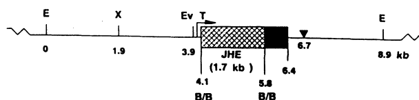
FIG. 1 Structure of the AcRP23.JHE virus. E, EcoRI sites; X, XhoI site; Ev, EcoRV site; B/B, BamHI/BglII ligation; T, transcription start site. The hatched area shows the coding region of JHE and the dark area the remaining polyhedron sequence.
