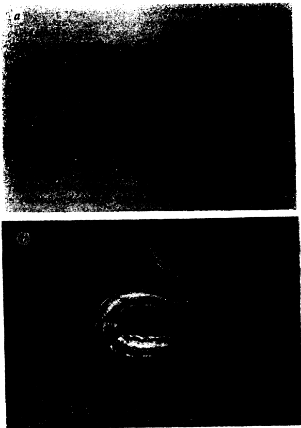
FIG. 3 The effects of expressed JHE on insects. a, The effects of JHE injected into mid-second instar larvae of M. sexta . b, The effects of infection of first instar larvae of T. ni with AcRP23.JHE.
