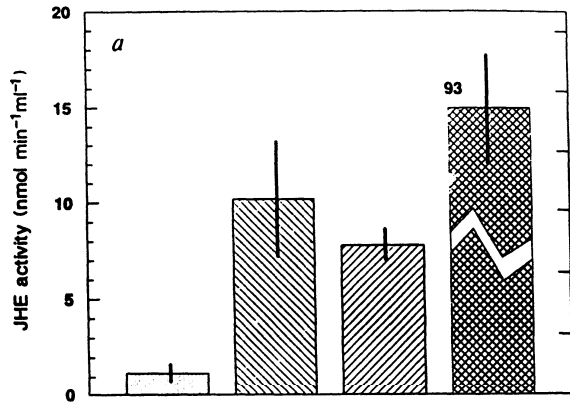
FIG. 4 The effects of AcRP23.JHE on larvae of T. ni . a , The effects of AcRP23.JHE infection on haemolymph JHE levels in T. ni . Following infection as described below, individual larvae were bled when the control larvae were in the third instar. The first bar indicates the low levels of JHE seen in the mid-third instar of feeding animals (or in larvae infected with wild-type AcNPV or AcNPV containing the gp120 gene 23 ). The second bar indicates the much higher levels of JHE found in infected larvae, whereas the third bar shows the JHE levels in 10 control insects at 'bubble head' (the time between head capsule slippage and ecdysis). For comparison, the fourth bar (note different scale on right) shows the level of JHE present at peak levels in the normal fifth instar (the average rate of hydrolysis is indicated above it). b , Minimum, maximum and median weights of larvae exposed to AcRP23.JHE as first stadium larvae. Median weights are shown because some insects are not infected at lower doses. The mean weights of animals
