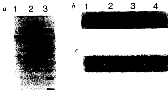
FIG. 2 Analysis of JHE purified by affinity chromatography from the haemolymph of fifth instar larvae of H. virescens and from the growth medium of cells of S. frugiperda infected with AcRP23.JHE. a Sodium dodecyl sulphate polyacrylamide gel electrophoresis on a 12% gel stained with Coomassie Blue reveals slight differences in relative molecular mass ( M_r ). Lane 1, 2 \mu\text{g} of JHE expressed by the recombinant baculovirus (66K); lane 2, 2 \mu\text{g} of JHE from haemolymph (62K); lane 3, M_r standards of 97, 67, 43, 31, 22 and 14K. The data from a western blot (b) and a glycan blot (c) demonstrate that the difference in M_r is due to differential glycosylation of JHE. The central lanes show the effects of digestion with an endoglycosidase. b, c Lanes 1, undigested JHE from recombinant baculovirus; lanes 2, digested JHE from recombinant baculovirus; lanes 3, undigested JHE from haemolymph; lanes 4, digested JHE from haemolymph. In (b), the two digested preparations showed shifts to identical mobility. The immunologic similarity between the two purified preparations was revealed when the filter was probed with polyclonal antibodies developed against JHE from haemolymph 7 . In (c), the digested proteins lost their glycan-staining ability when they were treated according to the instructions of a glycan-staining kit 17 , showing that all oligosaccharides had been removed. METHODS. The two purified preparations were digested with an endoglycosidase selective for N-linked oligosaccharides (Peptide:N-acetylglucosidase F, Boehringer Mannheim Biochemicals) and analysed by immunoblotting (b) and blotting specifically for glycans (c) on proteins transferred to nitrocellulose filters by standard procedures. Gels b and c were run for 90 rather than 60 min and the bands of interest were enlarged to emphasize differences in M_r .
