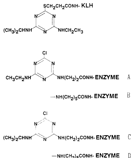
Figure 1. KLH conjugate and the hapten-enzyme conjugates. Two simazine tracers (A and B) and two atrazine tracers (C and D), each with a short \text{C}_3 or a long \text{C}_6 handle, were conjugated. The haptens were attached via their carboxyl groups to the amino groups of the enzymes. Additionally presented is the atrazine thiopropionic acid, which was coupled to hemocyanin from keyhole limpet (KLH) for immunization (Goodrow et al., 1990).
