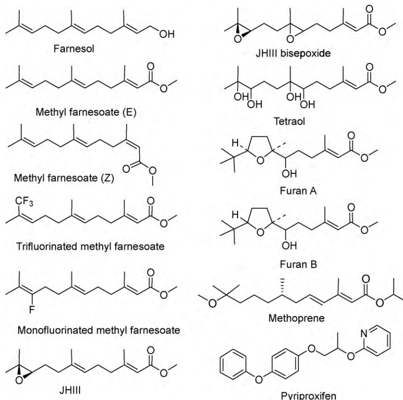
Fig. 1. Chemical structures of tested compounds.
