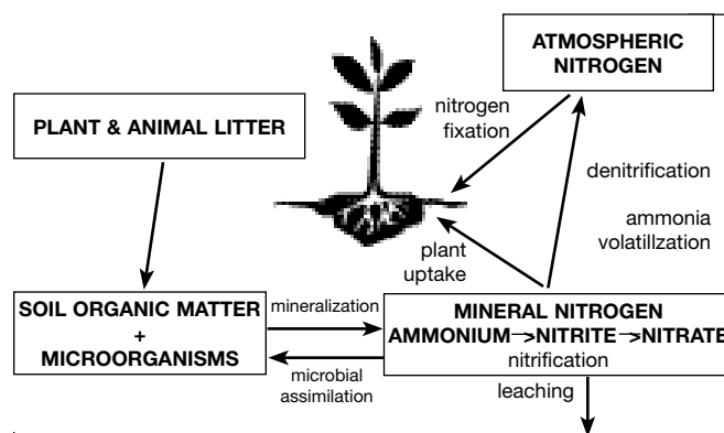
Figure 4-1. Nitrogen cycling (adapted from Chaney, Drinkwater, and Pettygrove 1992).
