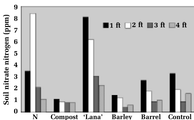
Figure 4-3. Effect of cover crop on soil nitrate-nitrogen in a Thompson Seedless vineyard in the San Joaquin Valley, June 1992.
