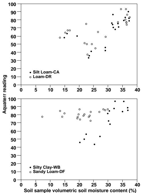
Fig. 2. Aquaterr readings versus soil sample moisture contents for four locations.
