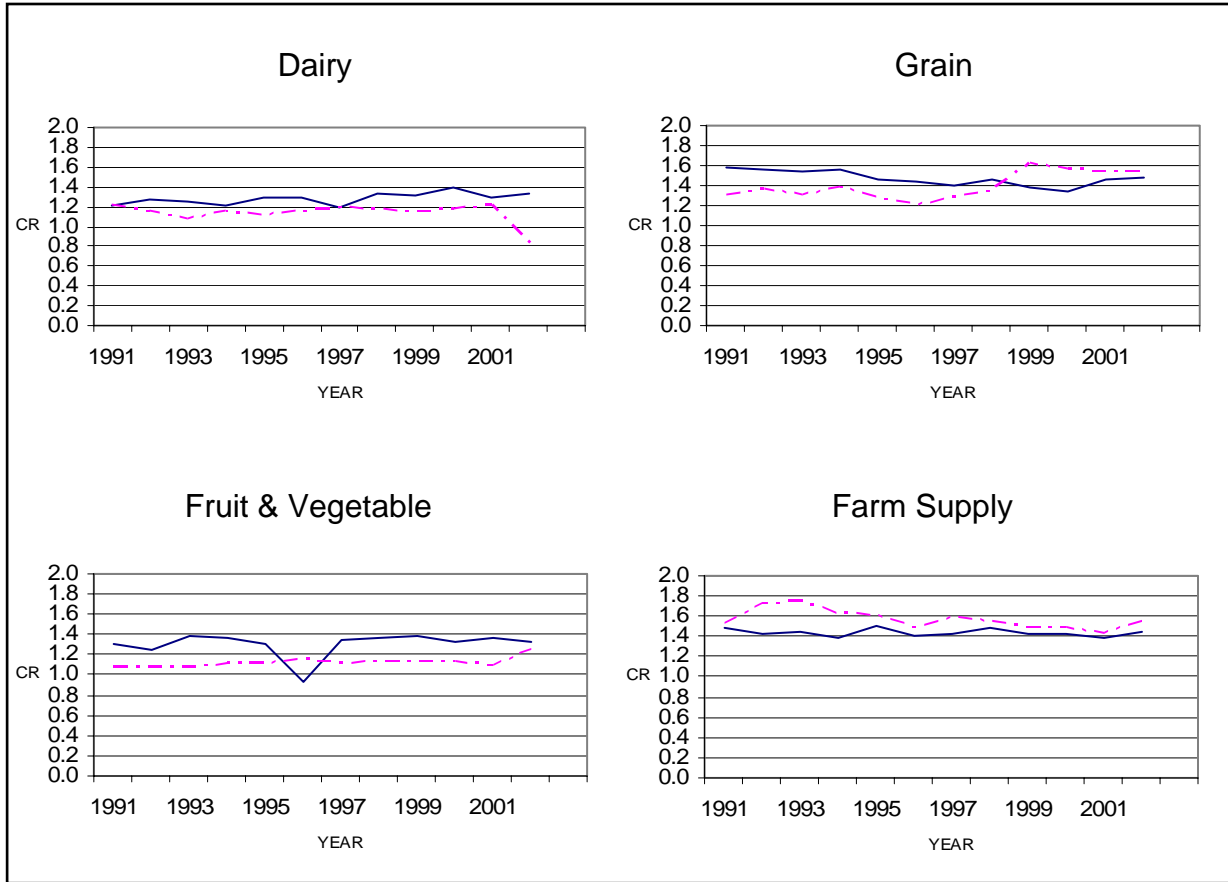
Figure 4. Current ratio
