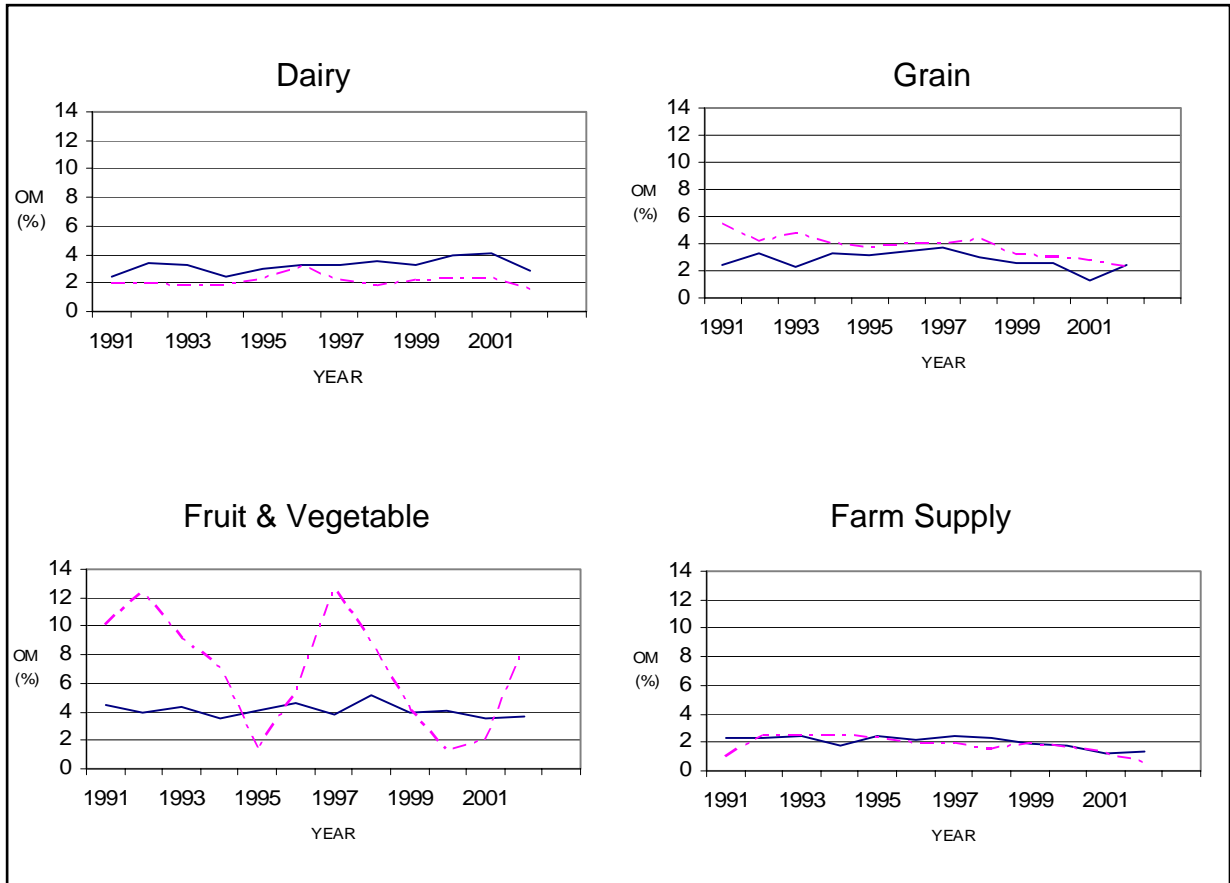
Figure 3. Operating margin
