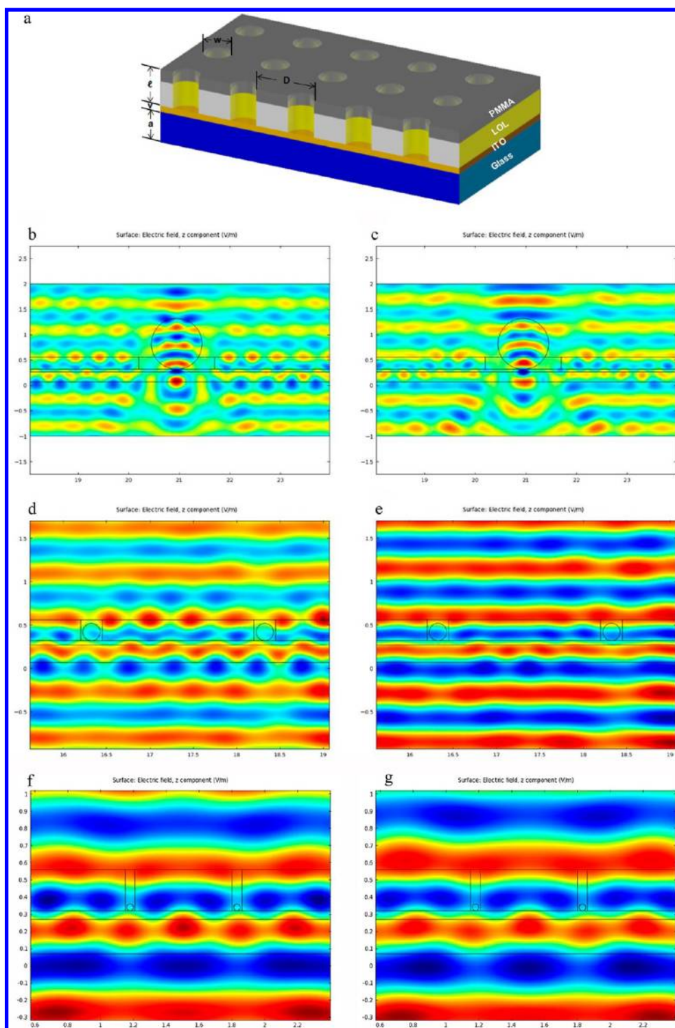
Figure 3. Numerical modeling of the nanoarray with PC structure. (a) 3-D geometry of the nanoarray; W/D : 60 nm/650 nm (40 nm particle), 250 nm/2 \mu\text{m} (200 nm particle), 1.5 \mu\text{m}/10 \mu\text{m} (1 \mu\text{m} particle), 7 \mu\text{m}/0 \mu\text{m} (5 \mu\text{m} particle); v : 50 nm; z : 240 nm (85 nm PMMA and 155 nm LOL; PMMA and LOL 2000 were assumed to be single layer in the model), a : 1.1 mm, (b) spatial distribution of the electric field intensity confined within 1 \mu\text{m} PC-microarray for 532 nm wavelength, (c) 1 \mu\text{m} PC-microarray for 555 nm wavelength, (d) 200 nm PC-nanoarray for 532 nm, (e) 200 nm PC-nanoarray for 555 nm, (f) 40 nm PC-nanoarray with 650 nm eriodicity for 532 nm, (g) 40 nm PC-nanoarray with 650 nm periodicity for 555 nm.
